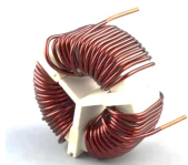
交流共模滤波器 (三相) AC Common mode Choke Coil (Three phase)
